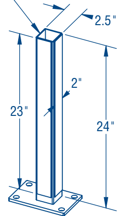
Gate Shoe
